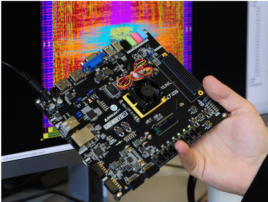
Figure 7. The Digilent Genesys 2 Xilinx FPGA board that has PULPissimo images ready to be used. The same board is also targeted by the CVA6/Ariane platform described under Section 3.3.2
