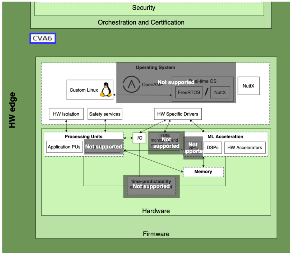
Figure 14 CVA6 as part of the FRACTAL big picture
