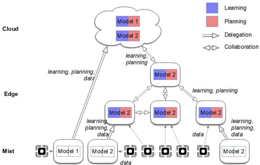
Figure 3. A schematic drawing of a possible FRACTAL system deployment using three different tiers of FRACTAL hardware nodes with different capabilities (drawing from WP5 technical meetings).
