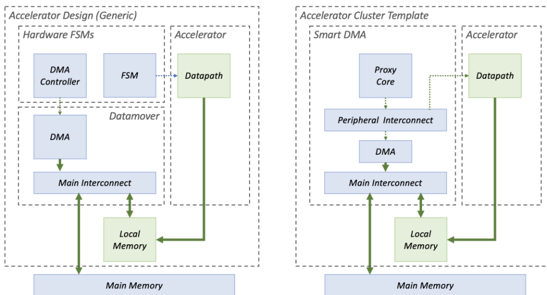
Figure 15 Accelerator Design Options
