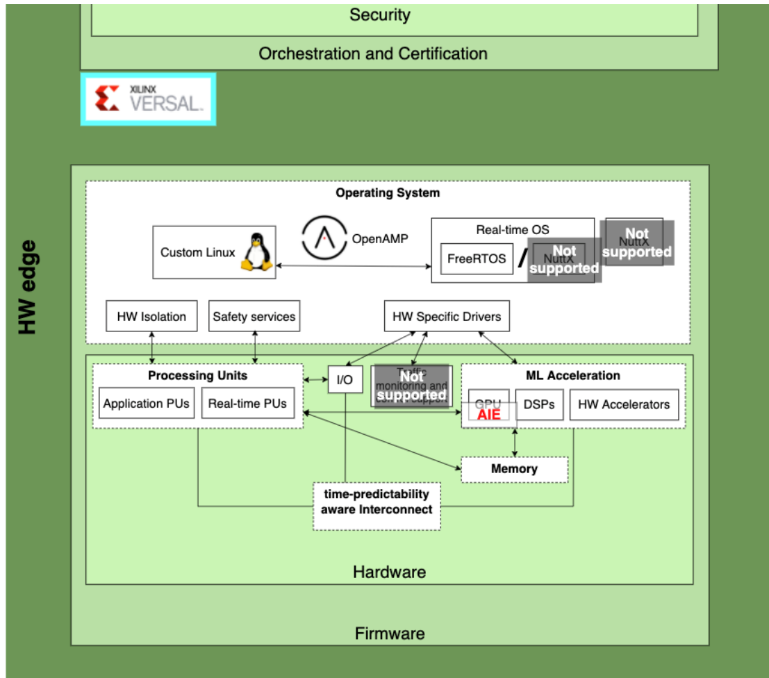
Figure 6 The VERSAL platform in the FRACTAL big picture
