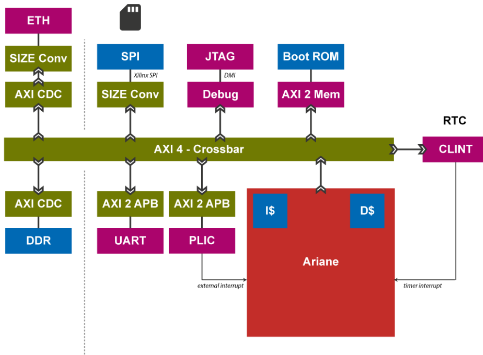
Figure 13: Schematic of the Ariane/CVA core mapped to the Genesys 2 board.
