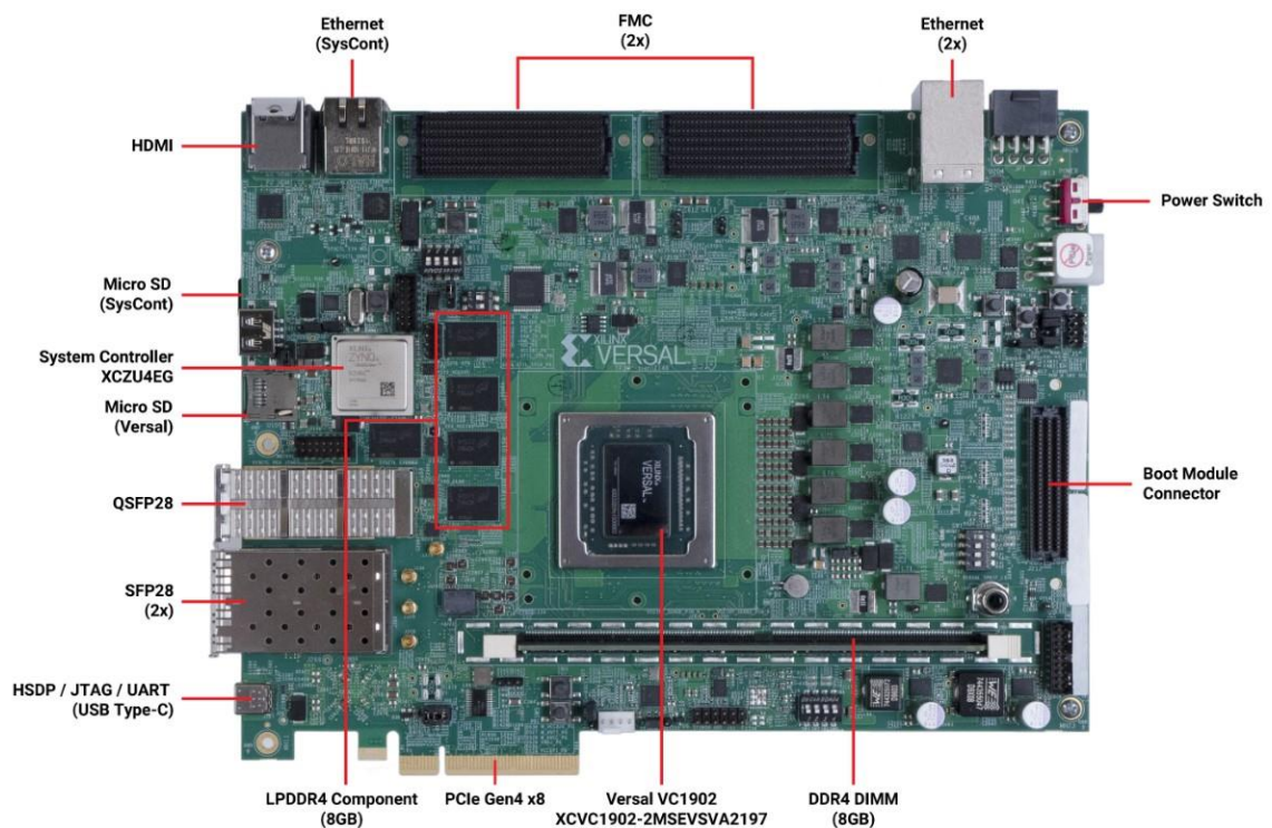
Figure 5. The Versal AI Core Series VCK190 Evaluation Kit
