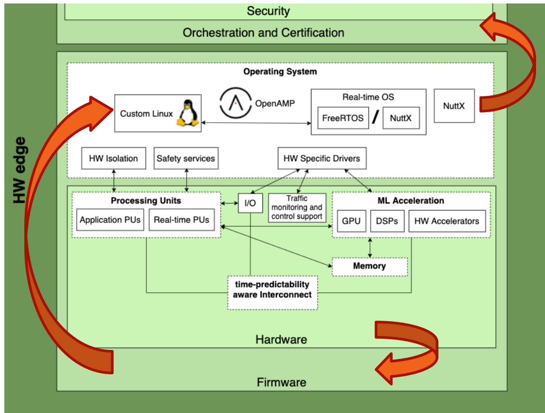
Figure 2 The hardware node part of the Big Picture for FRACTAL. To adapt to the overall FRACTAL description, this part of the graph has been layered differently and arrows have been added to guide the viewer that are familiar with a more traditional view that orders hardware, firmware, software
