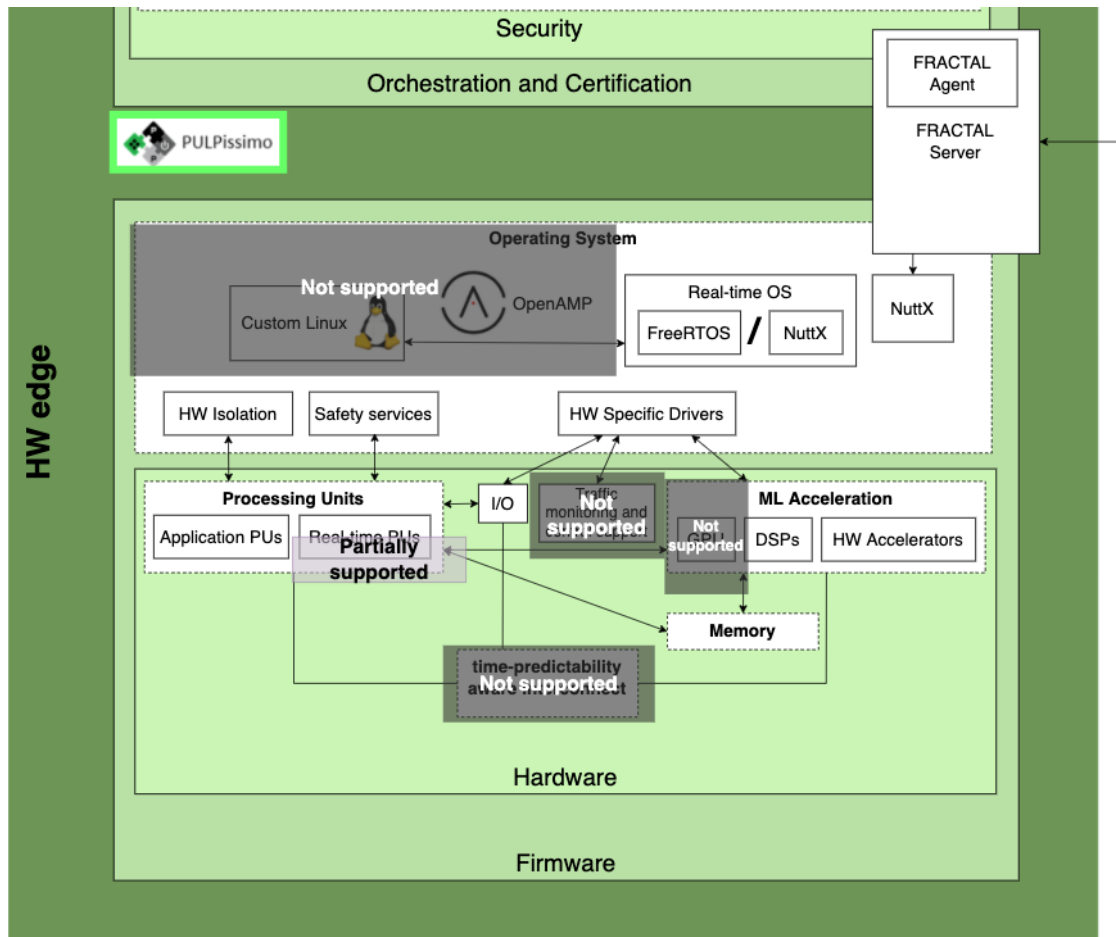
Figure 10 PULPissimo as part of the FRACTAL big picture
