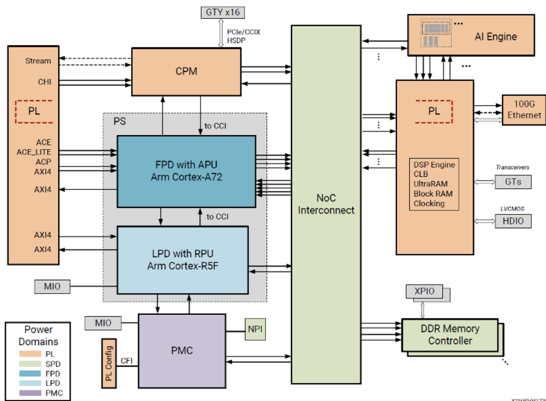
Figure 4. Top level schematic of Xilinx VERSAL Platform
