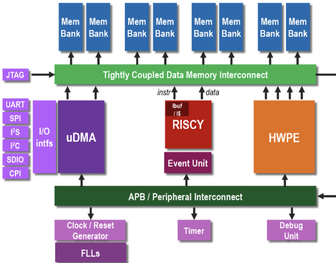
Figure 8. Block diagram of the PULPissimo system using a single 32bit RISC-V core (RI5CY/CV32E40P) and can easily be extended with accelerators, APB/AXI peripherals as well as instruction set extensions.
